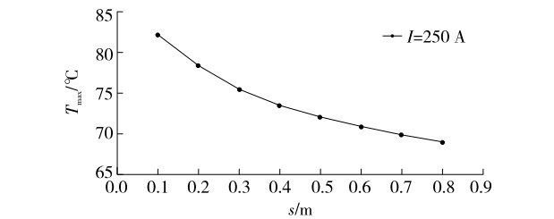
图 16 支架层间距对双根电缆运行最大温度 T_{\max} 的影响 Figure 16 Influence diagram of bracket spacing on the maximum operating temperature T_{\max} of two cables
