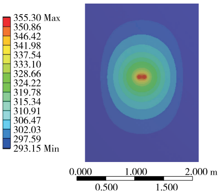
图 7 双根电缆温度场分布云 Figure 7 Double cables temperature field distribution cloud map
