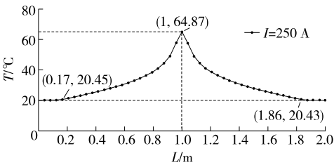
图 6 单根电缆温度场分布 Figure 6 Temperature distribution diagram of single cable
