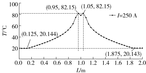
图 9 双根电缆温度场分布 Figure 9 Temperature field distribution diagram of two cables
