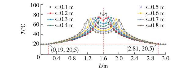
图 15 支架层间距对电缆温度场分布影响 Figure 15 Influence diagram of bracket spacing s on cable temperature field distribution
