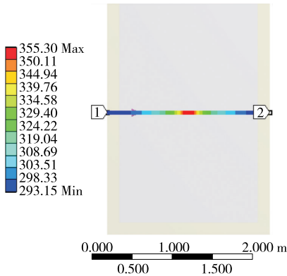
图 8 双根电缆温度场随路径分布云 Figure 8 Cloud image of temperature field distribution of two cables along the path
