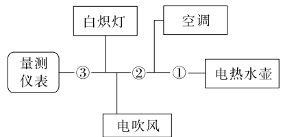
图 4 故障实验场景 Figure 4 Schematic diagram of the fault experiment scenario
