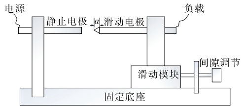
图 3 故障电弧发生装置 Figure 3 Fault arc generator
