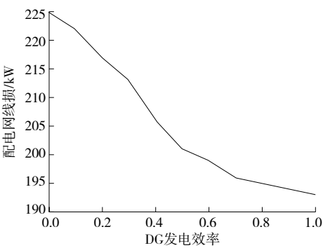
图 5 DG 典型日实际发电量比例对配网线损的影响 Figure 5 The influence of daily generation hour utilization on the distribution line loss
