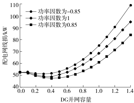
图 6 DG 运行功率因数对配电网线损的影响 Figure 6 Influence of DG operation power factor on the line loss of distribution network
