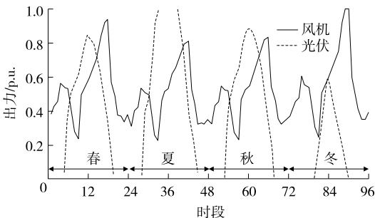
图 4 DG 各季度典型日出力波动曲线 Figure 4 Typical daily output fluctuation curve of DG in each quarter
