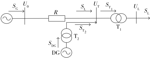
图 1 DG 并网后的单条馈线配电网理想拓扑 Figure 1 Ideal topology of single feeder distribution network with transformer parameters DG connected to power grid
