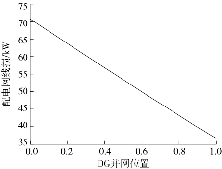
图 3 DG 并网位置对配电网线损的影响 Figure 3 Influence of DG grid connection position on the line loss of distribution network
