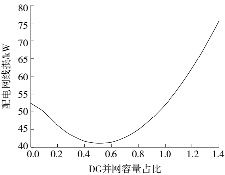
图 2 并网容量占比对配电网线损的影响 Figure 2 Influence of proportion of grid connected capacity on the line loss of distribution network
