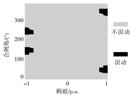
图 10 平衡剩磁下 20 kV 配电网线路零序过流保护的误动情况分布 Figure 10 Results of 20 kV distributing line zero-sequence over current protection when the three phase remanence is balanced
