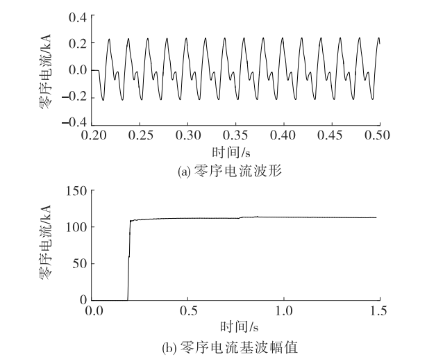
图 8 高压内置空载合闸期间 20 kV 线路零序电流波形 Figure 8 Zero-sequence current wave in a 20 kV line after the transformer is no-load energized
