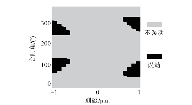
图 9 非平衡剩磁下 20 kV 配电网线路零序过流保护的動作情况分布 Figure 9 Results of 20 kV distributing line zero-sequence over-current protection when the three phase remanence is unbalanced
