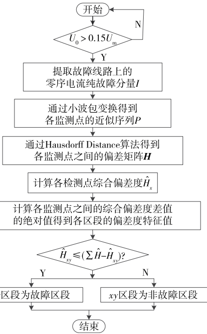
图 5 故障区段定位方法流程 Figure 5 Flow chart of fault section location method
