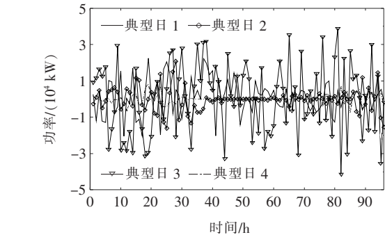
图 5 不同典型日的风电预测偏差量 Figure 5 Wind power forecast deviation of different typical days
