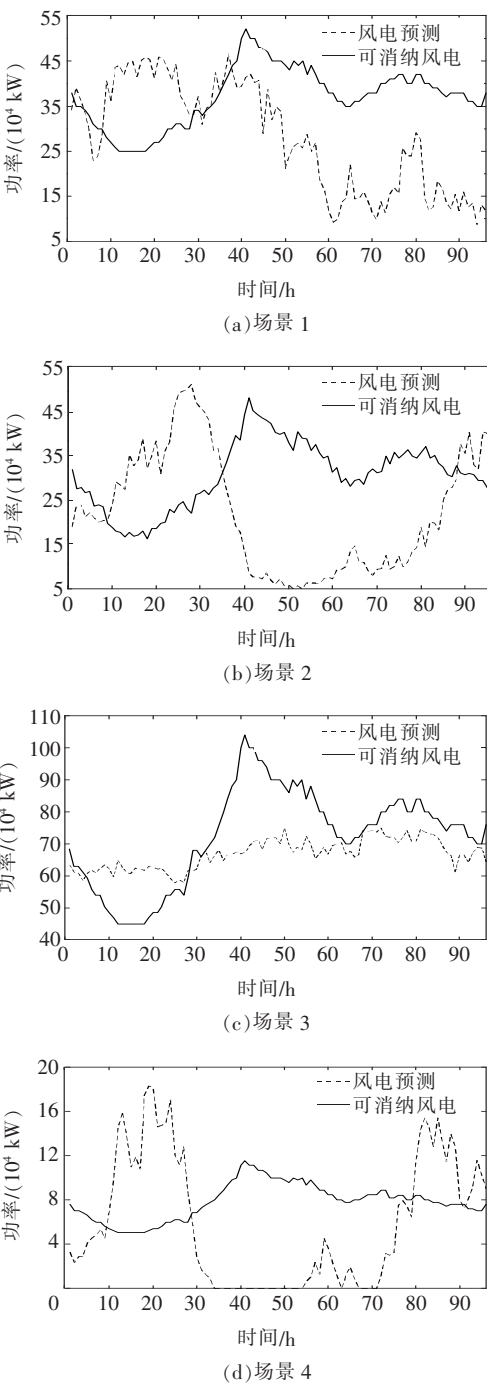
图 6 不同典型日的可消纳风电和预测出力 Figure 6 Different typical days can absorb wind power and forecast output
