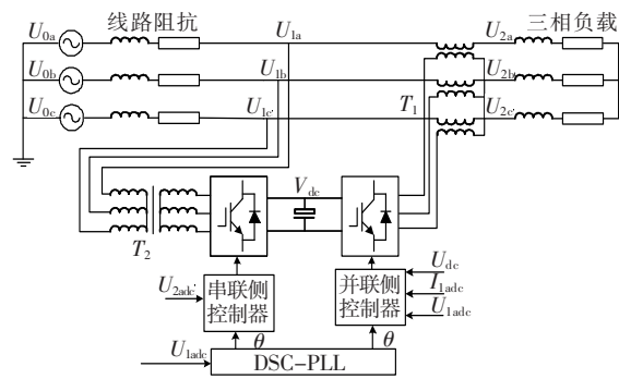
图 7 基于 PEVR 的电网电能质量治理仿真模型 Figure 7 Simulation model of power grid quality management based on PEVR
