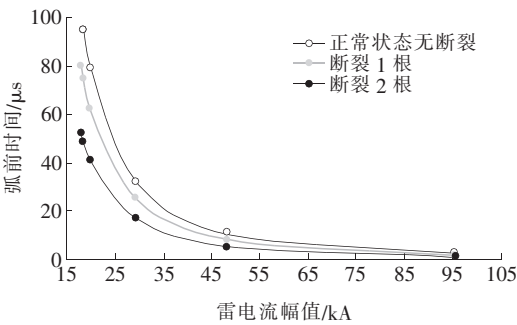
图 6 不同熔体断裂数下熔断器雷电流 幅值—弧前时间对比 Figure 6 Comparison of melt lightning current amplitude-pre-arc time under different melt fracture numbers
