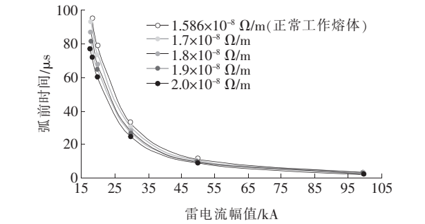
图 5 不同电阻率下熔断器雷电流幅值—弧前时间对比 Figure 5 Comparison graph of melt lightning current amplitude-pre-arc time under different resistivity
