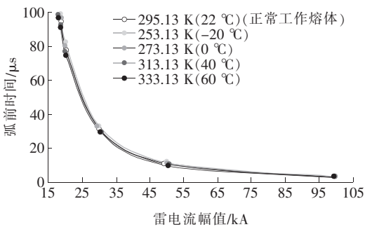
图 7 不同熔体环境温度下熔断器雷电 流幅值—弧前时间对比 Figure 7 Comparison of melt lightning current amplitude-pre-arc time at different melt ambient temperatures
