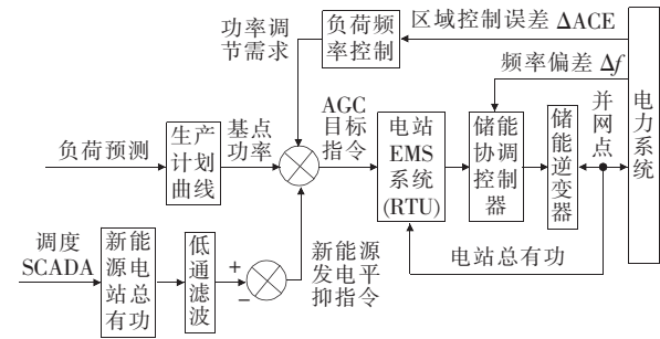
图 1 电网侧储能电站 AGC 控制总体结构框图 Figure 1 Structure diagram of AGC control of grid-side energy storage power station
