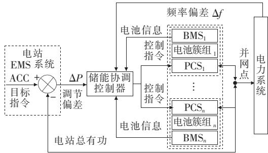
图 2 储能电站或单元参与电网频率控制原理 Figure 2 Schematic diagram of energy storage power station or unit participating in grid frequency control
