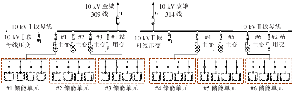
图 3 10 kV 雉城储能电站一次接线示意 Figure 3 Schematic diagram of the primary wiring of Zhicheng energy storage power station
