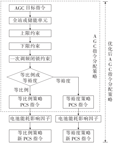
图 4 储能 AGC 控制策略(优化)指令计算流程 Figure 4 Energy storage AGC control strategy (optimization) instruction calculation flowchart
