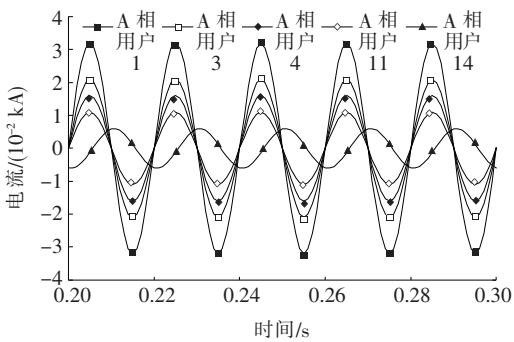
图 11 换相后 A 相各换相单元电流波形 Figure 11 Currents of phase A after commutation
