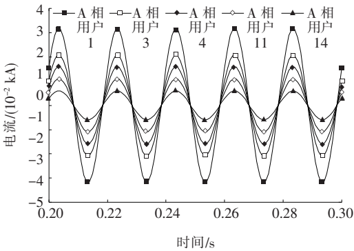
图 7 换相前 A 相各换相单元电流波形 Figure 7 Currents of Phase A before commutation
