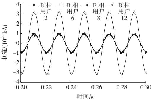
图 12 换相后 B 相各换相单元电流波形 Figure 12 Currents of phase B after commutation
