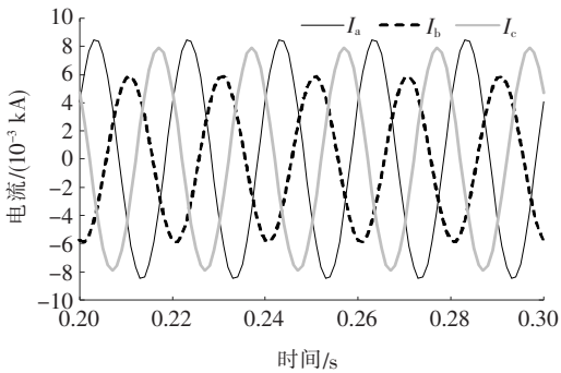
图 10 换相前三相电流波形 Figure 10 Three-phase currents before commutation
