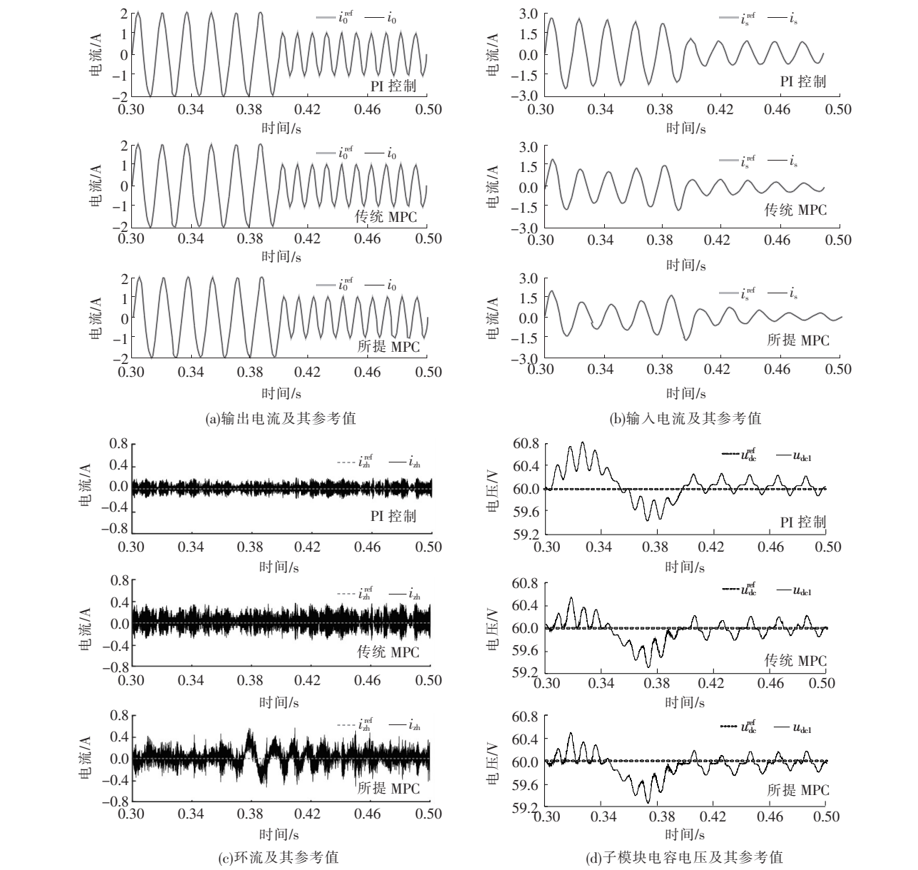
图 7 3 种控制策略仿真波形对比 Figure 7 Comparison simulation results with three strategies
