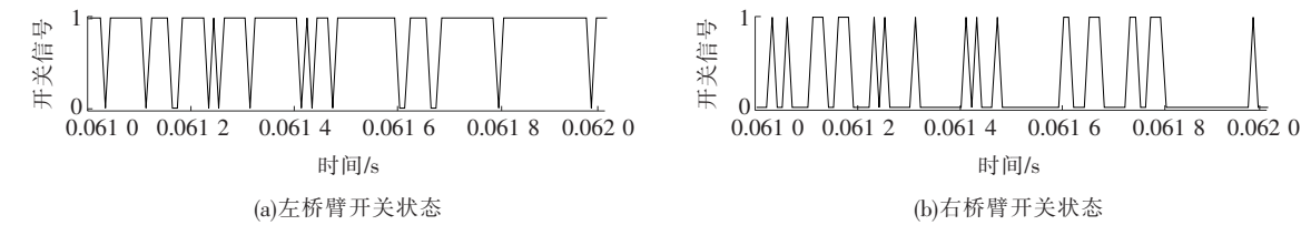
图 8 子模块左、右桥臂开关状态 Figure 8 Switching state of left and right arm of SM
