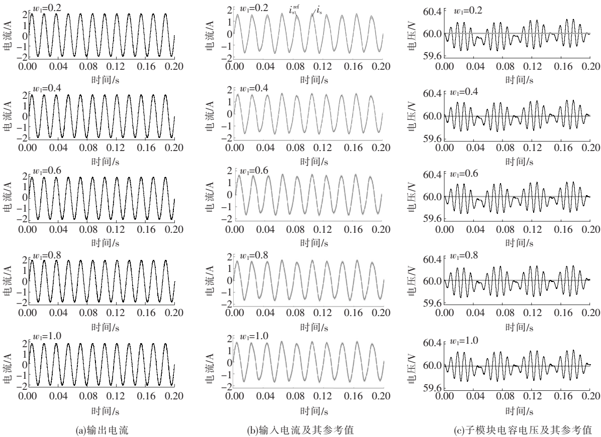
图 9 权重因子 w_1 变化时的仿真波形( w_2=1, w_3=0.2, w_4=0.8 ) Figure 9 Simulations when w_1 varies ( w_2=1, w_3=0.2, w_4=0.8 )
