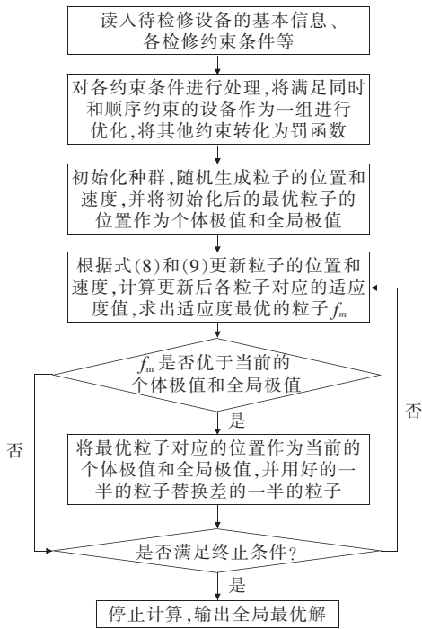
图 1 基于改进 PSO 的配网检修计划优化流程 Figure 1 Optimization process of distribution network maintenance plan based on Improved PSO
