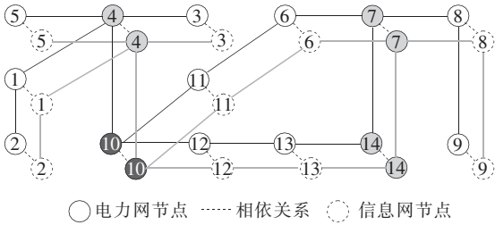
图 1 有电压等级信息网拓扑结构 Figure 1 Topology of information network with voltage level
