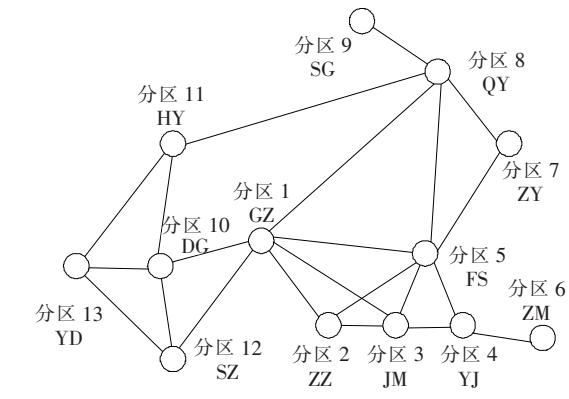
图 3 电网分区情况 Figure 3 Situation of power grid division
