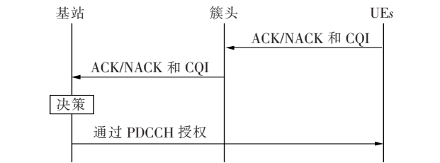
图 2 集中式重传的信令过程 Figure 2 Signaling process of centralized retransmission
