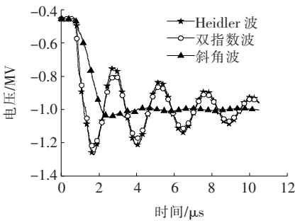
图 8 不同雷电流模型下断路器过电压波形 Figure 8 Overvoltage waveform of breaker under different lightning current models
