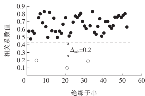
图 8 雨后相关系数散点分布 Figure 8 Spot diagram of correlation coefficients after rain
