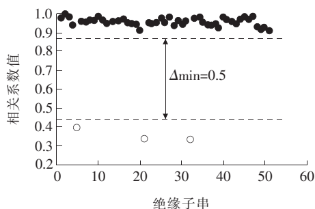
图 6 雨前相关系数散点分布 Figure 6 Spot diagram of correlation coefficients before rain
