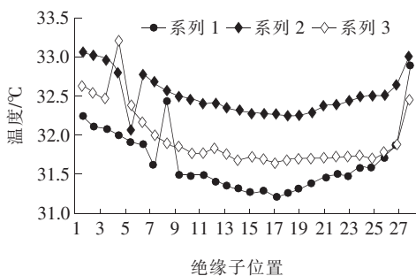
图 5 雨前含劣化绝缘子串温度分布曲线 Figure 5 Temperature distribution diagram of zero-valued insulator strings before rain
