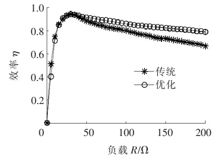
图 12 效率—负载特性曲线 Figure 12 Efficiency-load characteristics
