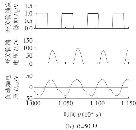
图 11 不同负载阻值时开关管电压波形 Figure 11 Waveform diagram of switch tube voltage under different load resistance
