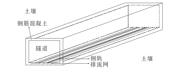
图 4 CDEGS 导体位置分布 Figure 4 Conductor position distribution diagram in CDEGS
