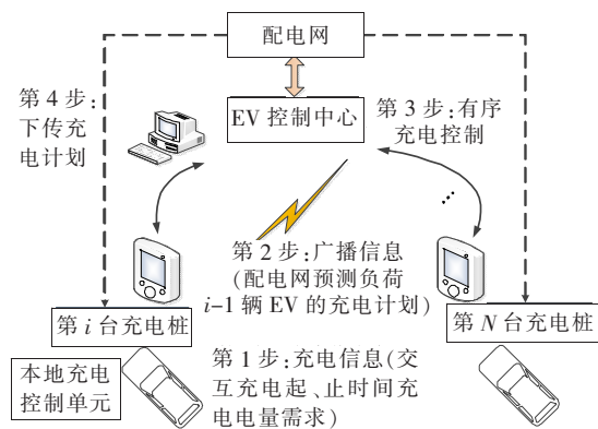
图 2 住宅小区电动汽车有序充电监控 Figure 2 Coordinated charging monitoring diagram of electric vehicles in residential quarters
