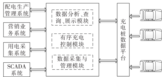
图 1 住宅小区电动汽车接入配电网的有序充电构架 Figure 1 Coordinated charging architecture diagram of residential quarter electric vehicles connected to the distribution network
