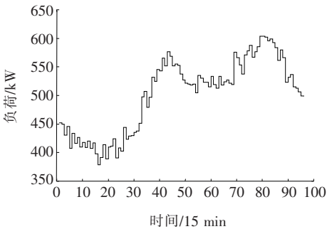
图 7 住宅小区负荷预测曲线 Figure 7 Residential district load prediction curve
