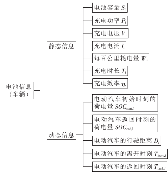
图 3 电动汽车电池信息采集 Figure 3 Electric vehicle battery information collection diagram
