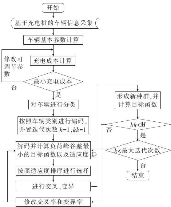
图 6 电动汽车有序充电的日前计划两阶段优化流程 Figure 6 Two-stage optimization flowchart of the day-ahead plan for coordinated charging of electric vehicles
