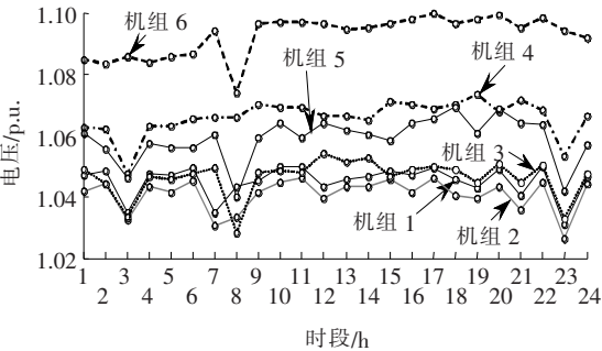
(b)机组机端电压
