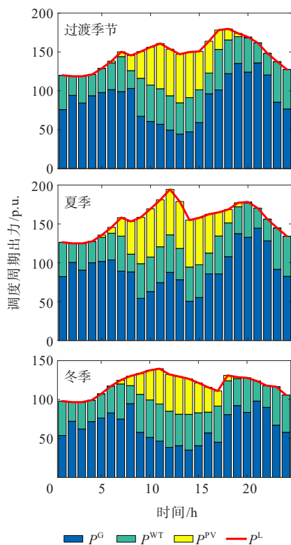
图4 过渡季节、夏季以及冬季典型日消纳结果 Figure 4 Absorptive results in typical day during the transition season, summer, and winter
