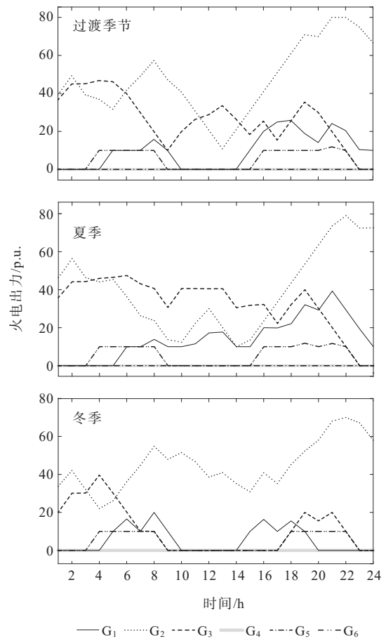
图5 过渡季节、夏季以及冬季典型日各发电机组出力曲线 Figure 5 Output curves of each generator unit in typical day during the transition season, summer, and winter
